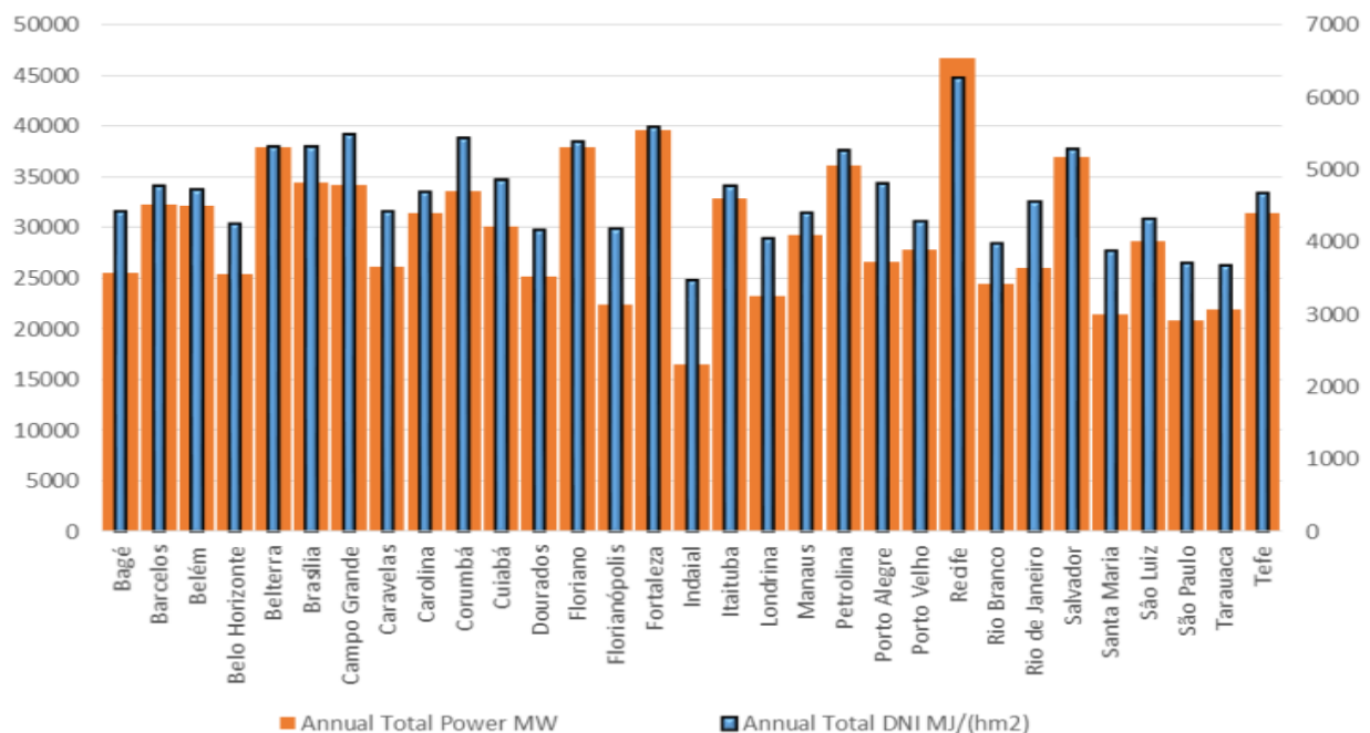
Figure 3: Annual total power and annual total solar resource by site location in Brazil
