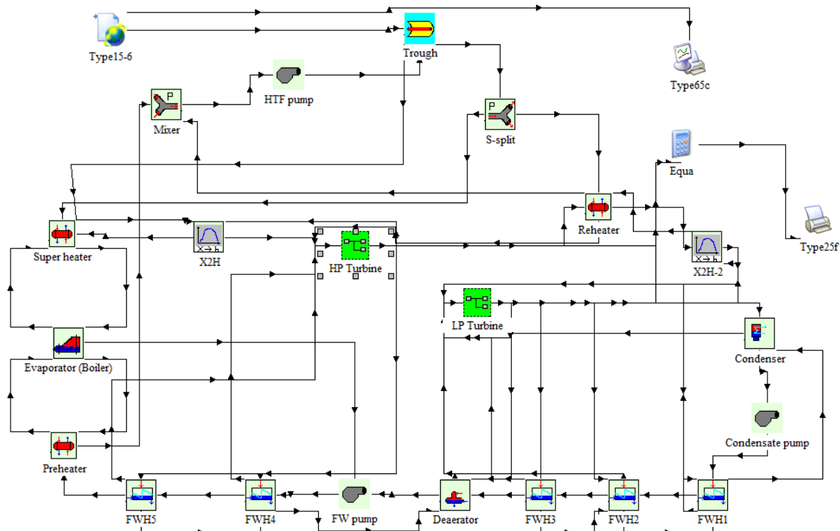
Figure 2: Simplified flow diagram of the Parabolic Trough Solar Plant
