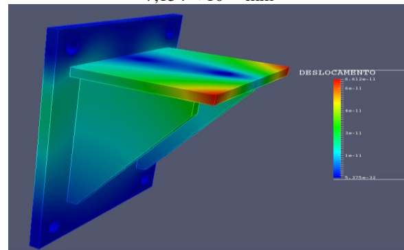
d) Code_Aster – Maximum value of displacement is 6,612 \times 10^{-02} mm
