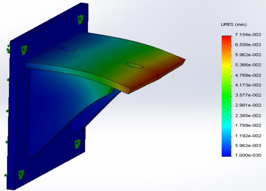
b) SolidWorks – Maximum value of displacement is 7,154 \times 10^{-02} mm
