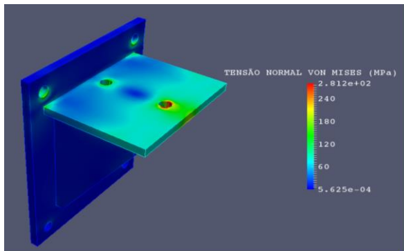
c) Code_Aster – Maximum value of Von Mises stress is 281,20 MPa
