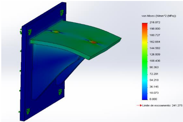
a) SolidWorks – Maximum value of Von Mises stress is 216,87 MPa
