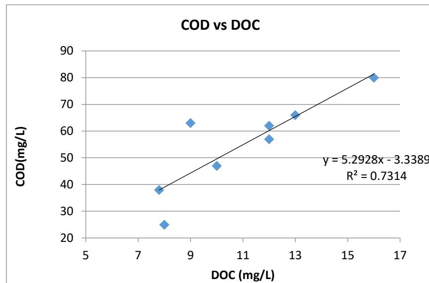
Figure 9: Correlation between COD vs DOC
