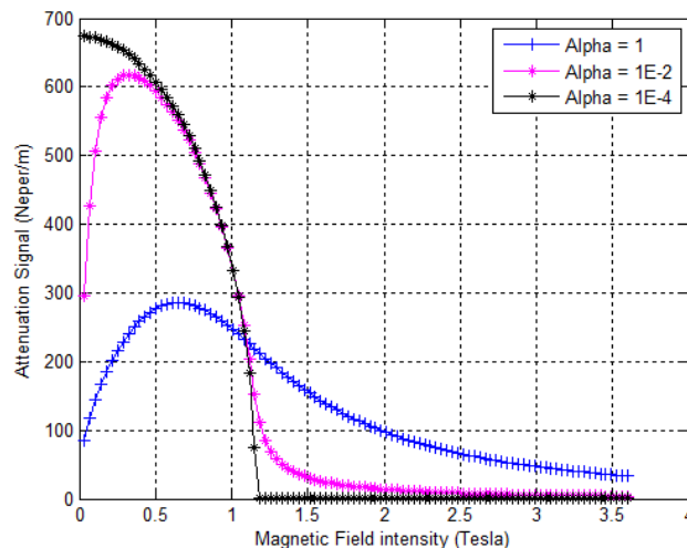
Figure 15: Attenuation signal versus magnetic field strength (Ka band)
