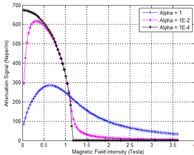
Figure 15: Attenuation signal versus magnetic field strength (Ka band)
