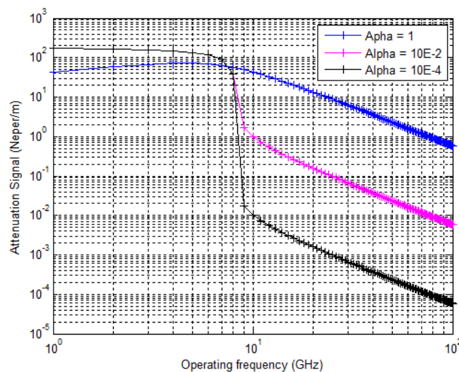
Figure 11: Attenuation signal ( N_e = 8.30 \times 10^{11} \text{ cm}^{-3} )
