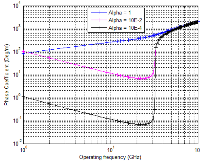
Figure 12: Phase coefficient ( N_e = 1.28 \times 10^{13} \text{ cm}^{-3} )
