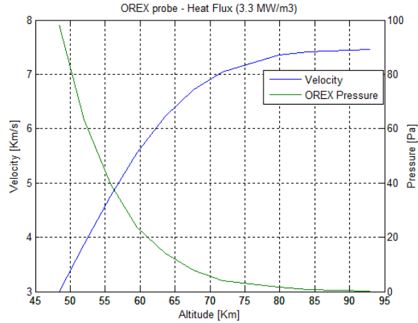
Figure 4: Variation of velocity and the pressure in function of the altitude for OREX probe
