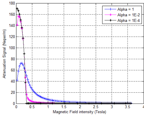
Figure 16: Attenuation signal versus magnetic field strength (X band)
