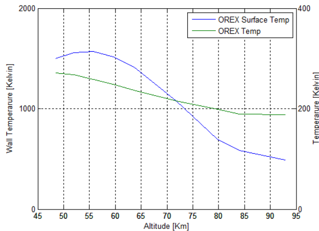
Figure 6: Variation of temperature in function the altitude for OREX probe
