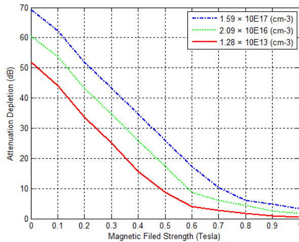
Figure 20: Attenuation reduction with SMF
