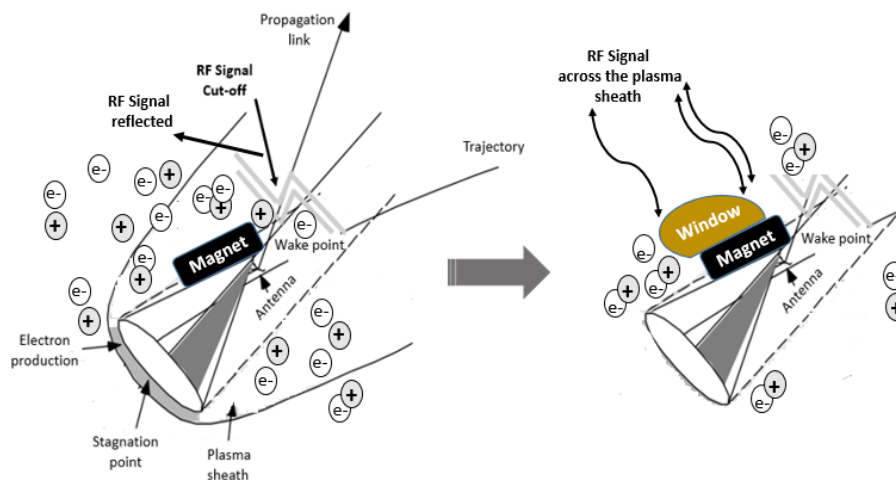
Figure 14: A Schematic of space probe including permanent magnet for mitigation method
