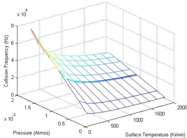
Figure 8: Collision plasma for ISAS data
