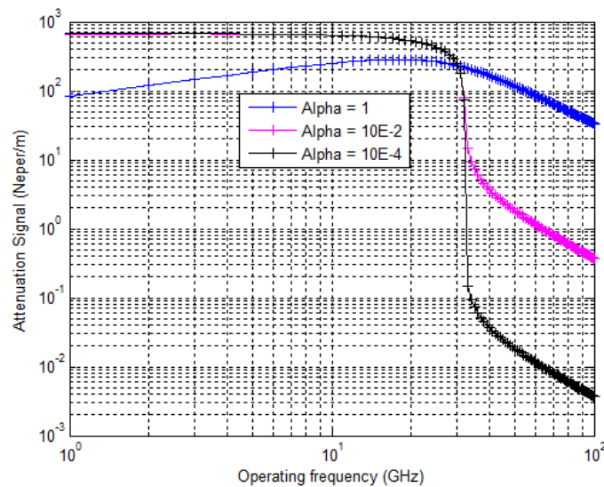
Figure 10: Attenuation signal ( N_e = 1.28 \times 10^{13} \text{ cm}^{-3} )
