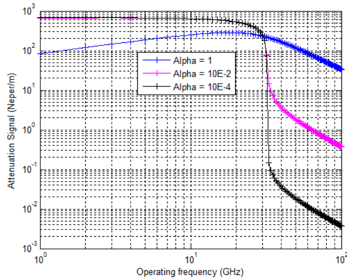
Figure 10: Attenuation signal ( N_e = 1.28 \times 10^{13} \text{ cm}^{-3} )
