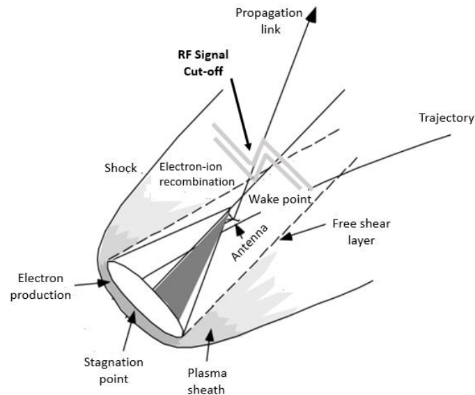
Figure 1: Space probe atmospheric entry.
