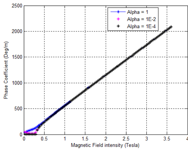
Figure 18: Phase shift versus magnetic field strength (X band)
