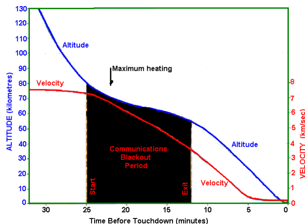
Figure 2: Typical space probe RF blackout reentry.
