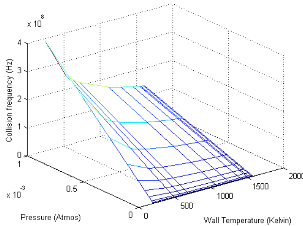
Figure 9: Collision plasma of OREX probe
