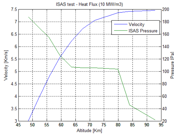
Figure 5: Variation of velocity and pressure in function of the altitude for ISAS test
