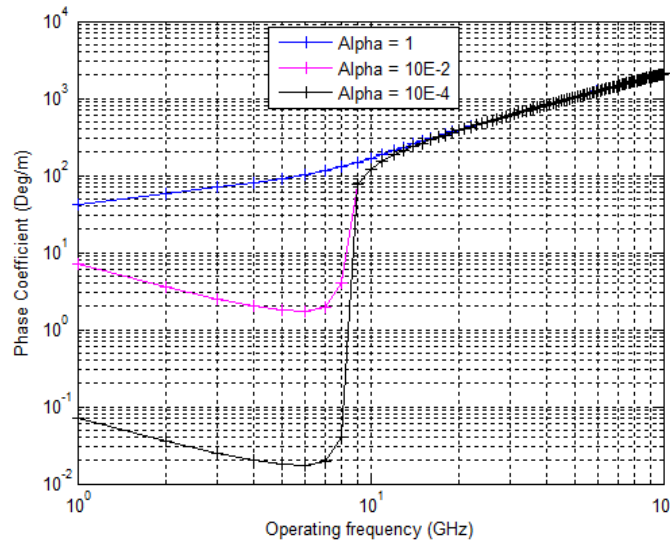
Figure 13: Phase coefficient ( N_e = 8.30 \times 10^{11} \text{ cm}^{-3} )
