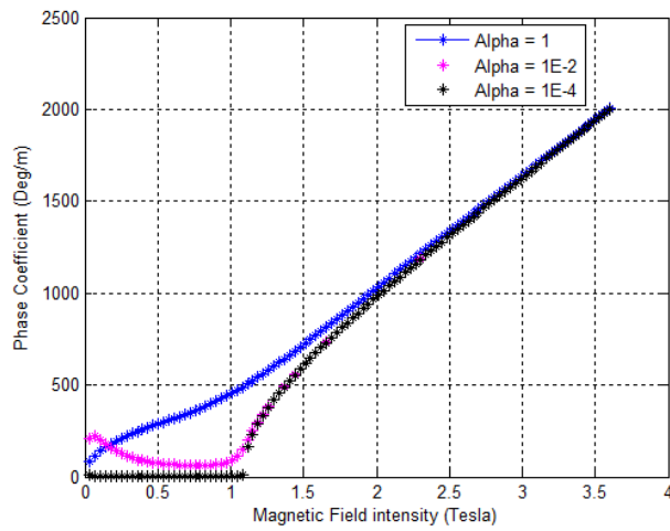
Figure 17: Phase shift versus magnetic field strength (Ka band)
