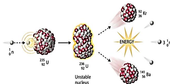
Figure 1: Fission reaction with {}_{92}\text{U}^{235}
